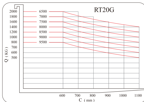
Load curve diagram
