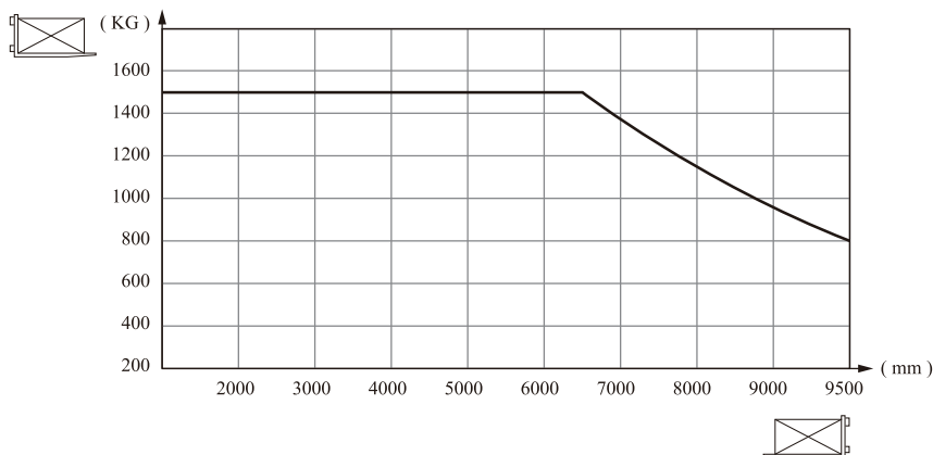
LIFTING HEIGHT-LOAD
