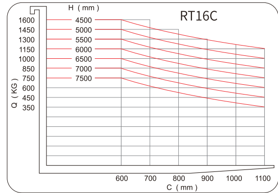
Load curve diagram
